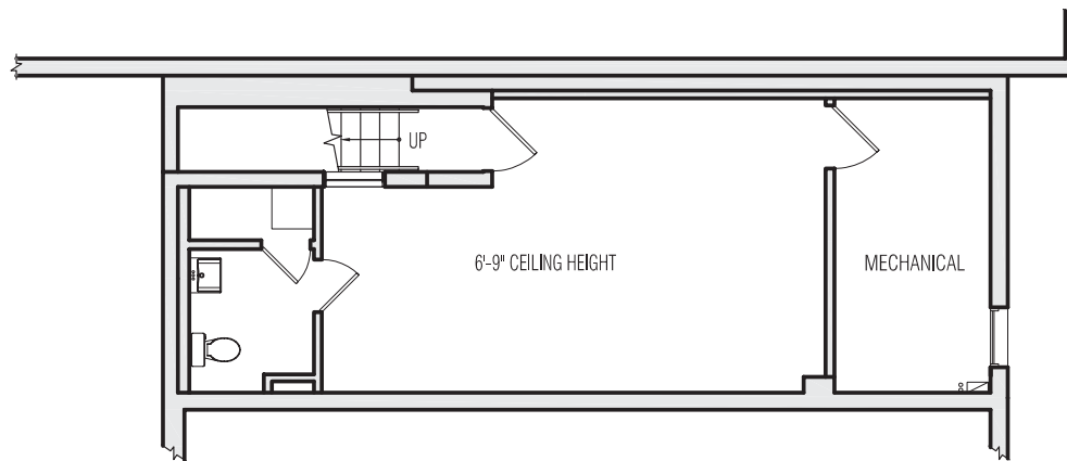
BASEMENT - 620 SF
