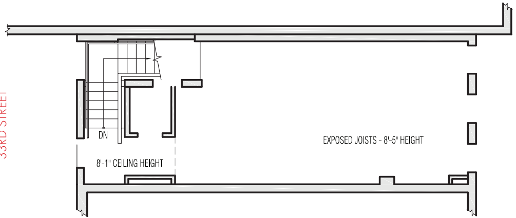
SECOND FLOOR - 620 SF
